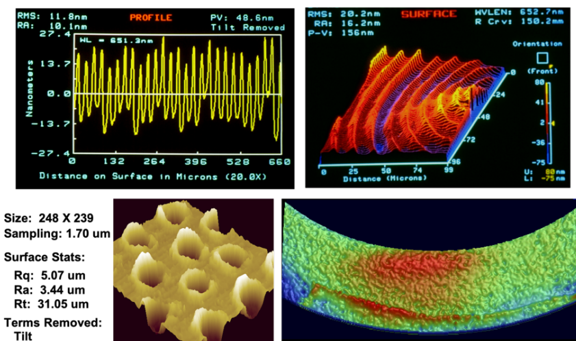
Fig. 12. (clockwise from top left) Diamond turned surface: Topo 2D and Topo 3D measurements. Stitched subregion of a fuel cap. Tiny pits in metal surface. (Photos courtesy of Kathy Creath and Jim Wyant).
