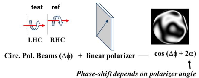
Fig. 15. Orthogonal circular polarization incident on a linear polarizer results in a variable phase shift between the two beams related to the angle of the linear polarizer. From [35].
