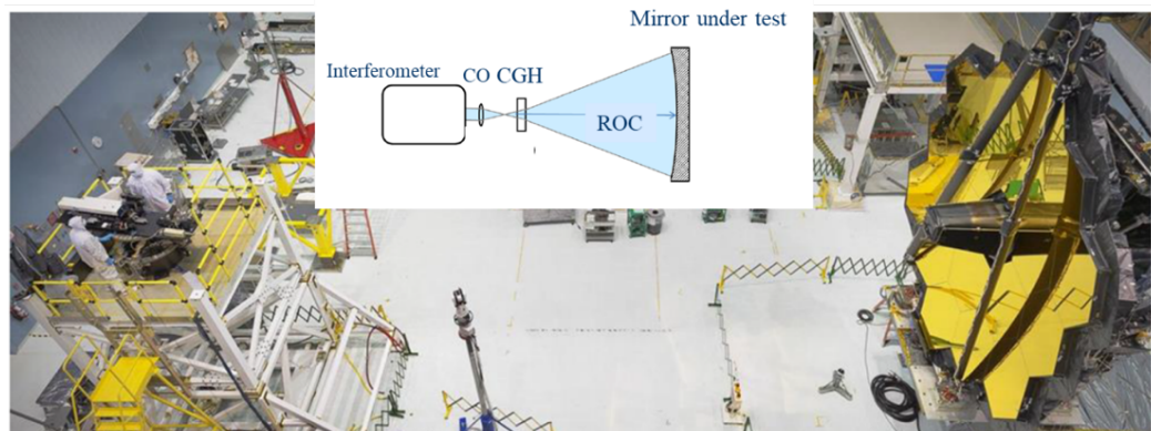
Fig. 19. Radius of curvature testing of the JWST [8].
